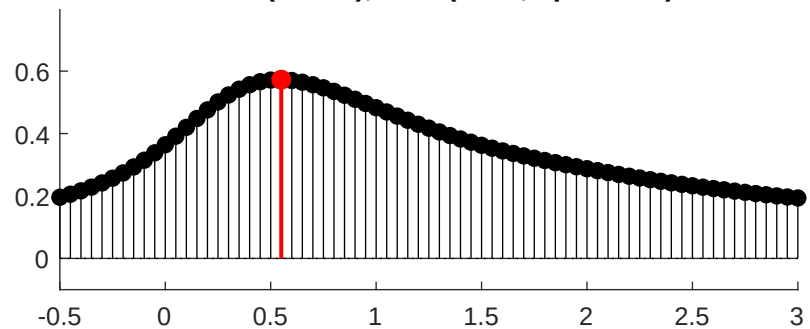
GRAB(DA2m), dark (n=19, opt=0.55s)
