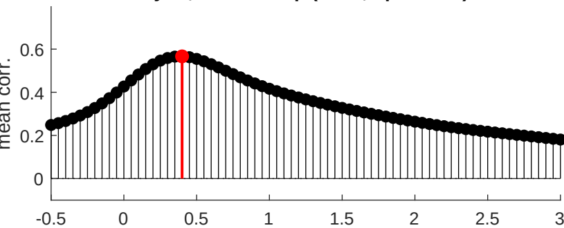
syt7f, closed loop (n=27, opt=0.40s)
