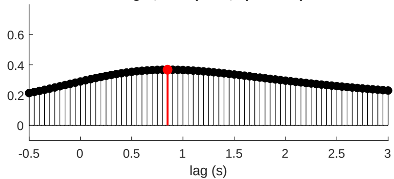
dLight, dark (n=25, opt=0.85s)
