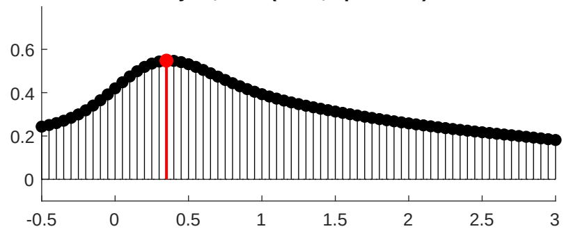
syt7f, dark (n=21, opt=0.35s)
