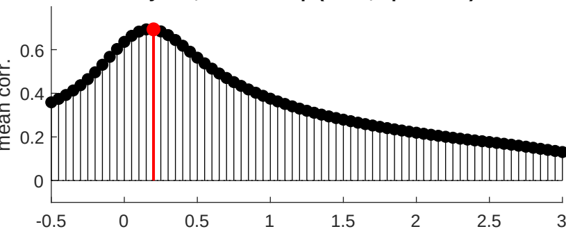
syt8m, closed loop (n=11, opt=0.20s)
