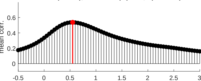
GRAB(DA2m), closed loop (n=17, opt=0.55s)
