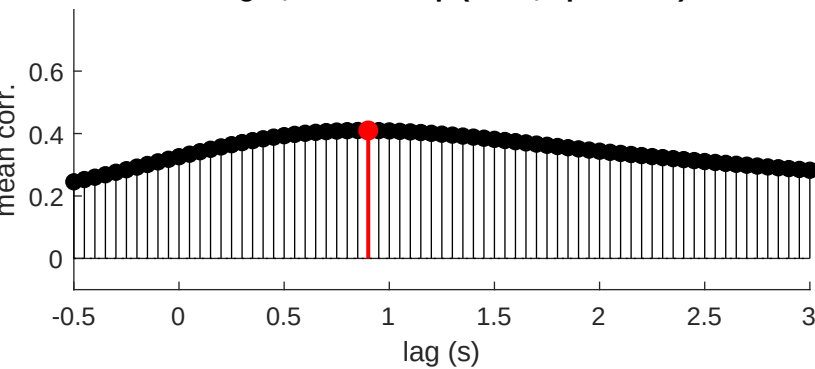
dLight, closed loop (n=71, opt=0.90s)
