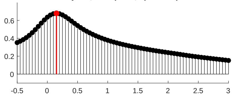
syt8m, dark (n=10, opt=0.15s)
